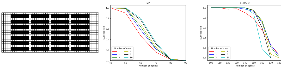
Figure 2: Left: Automated warehousing domain. Center and Right: Success rates of RRR strategies for M* and ECBS(2).
